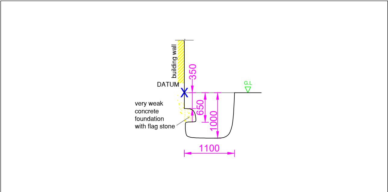
TRIAL PIT SECTION, 1:50 ON A4
