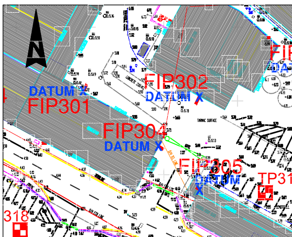
TRIAL PIT LOCATION PLAN, NTS on A4
