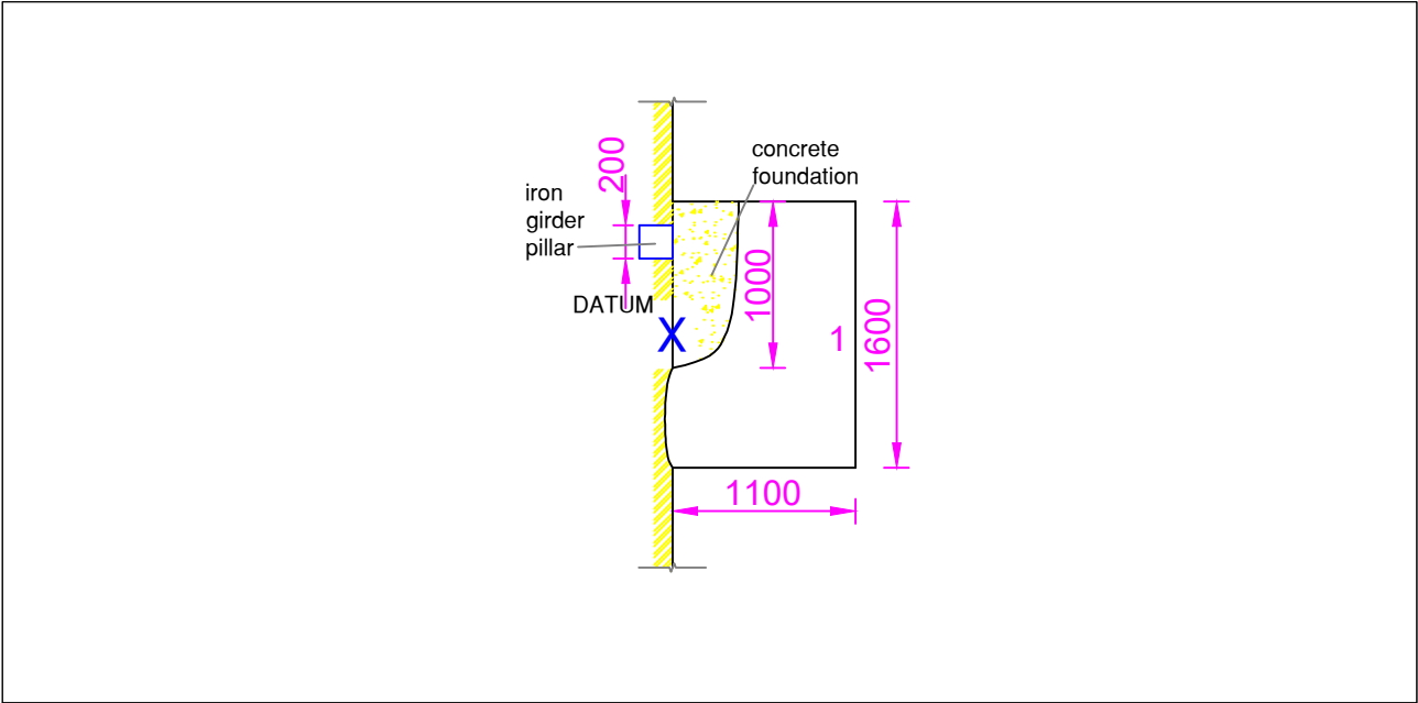
TRIAL PIT PLAN, 1:50 ON A4
